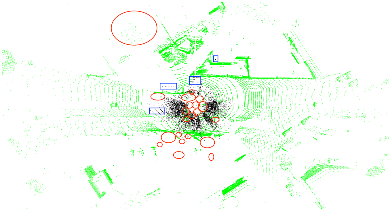
(b) SSR Thresholding at 2.5
